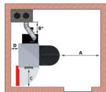
P4 Pellet with calorific value heat exchanger
